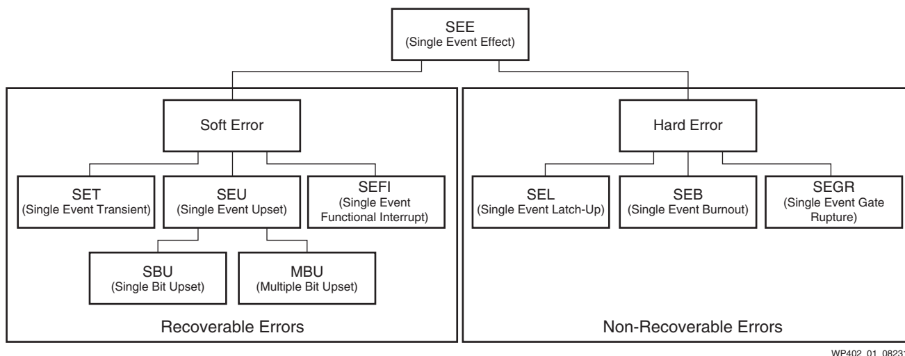
Figure 1: Types of Single Event Effects
