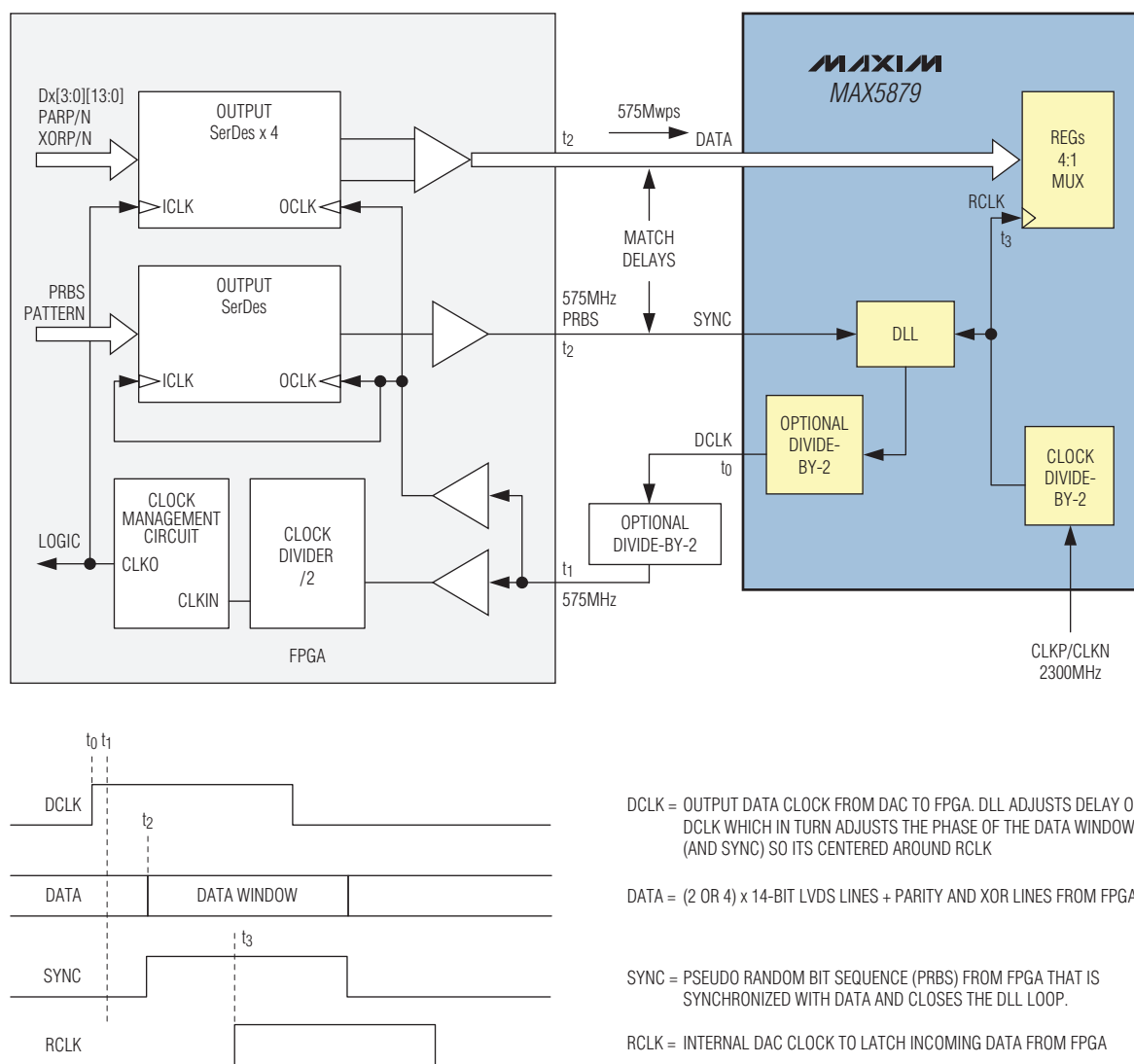
Figure 17. Digital Interface Between FPGA and the MAX5879 RF-DAC (in 4:1 Mux Mode)
