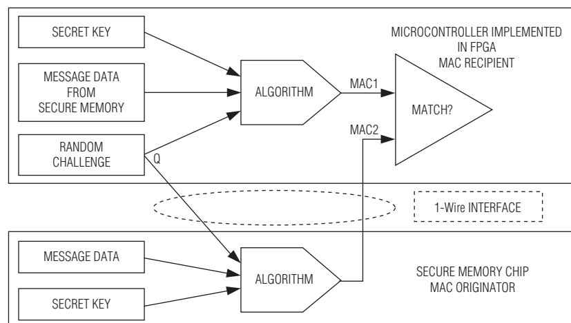
Figure 14. The Challenge and Response Authentication Process Proves the Authenticity of a MAC Originator
