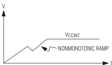
Figure 4. Nonmonotonic Startup Voltage Ramp
