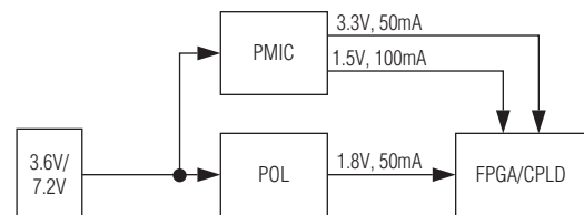
Figure 2. Typical FPGA Power Architecture Used in Communications, Industrial, and Consumer Applications
