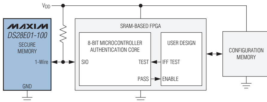
Figure 15. In This Simplified Schematic, a Secure 1-Wire Memory is Used for FPGA Protection
