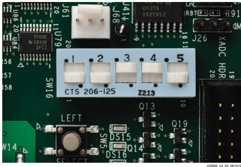
Figure 3-3: Switch Settings for the Mode Switch to Boot from the SD-MMC Card
