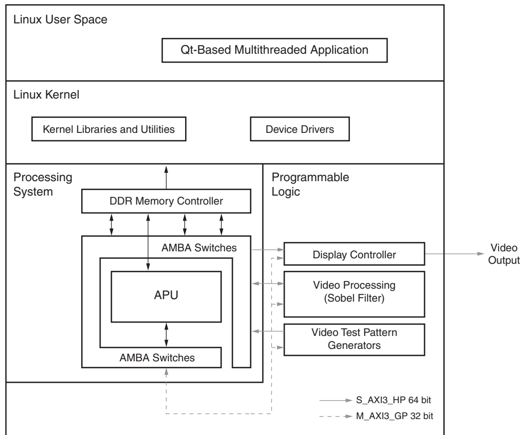
Figure 3-1: Zynq-7000 EPP Base TRD System Block Diagram
