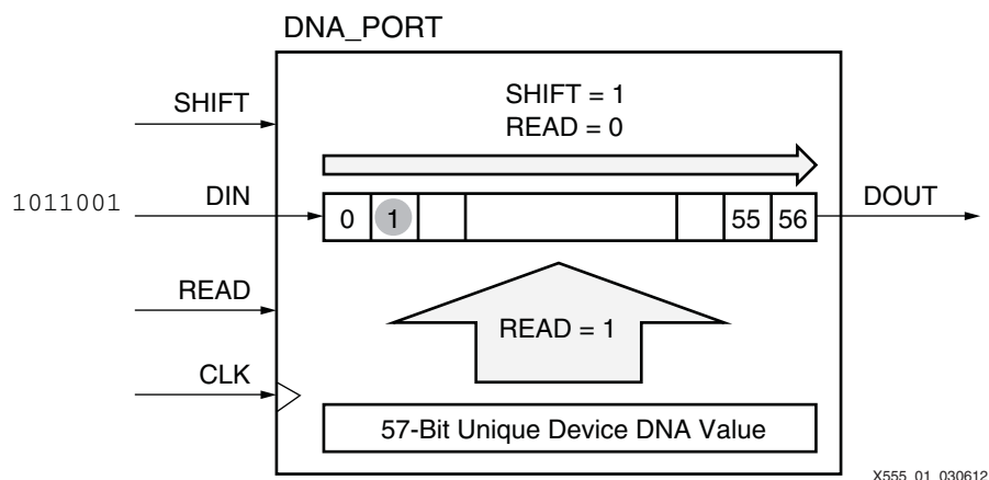
Figure 1: Extracting the Voltage Identification Bit from Device DNA
