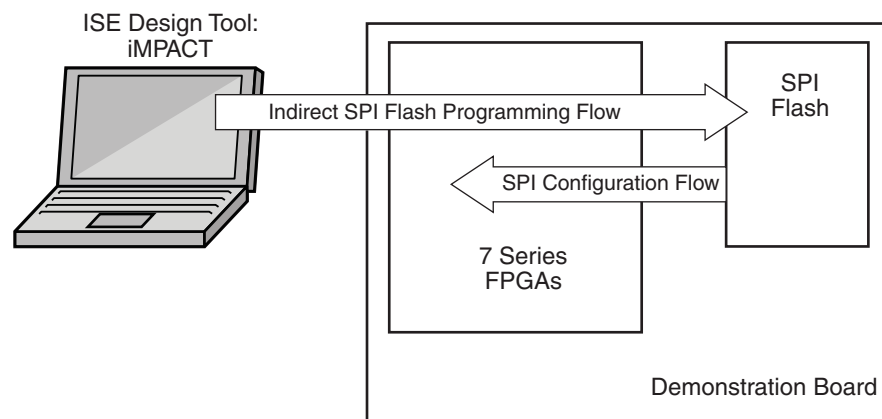
Figure 1: SPI Flash Configuration and Indirect Programming Flows
