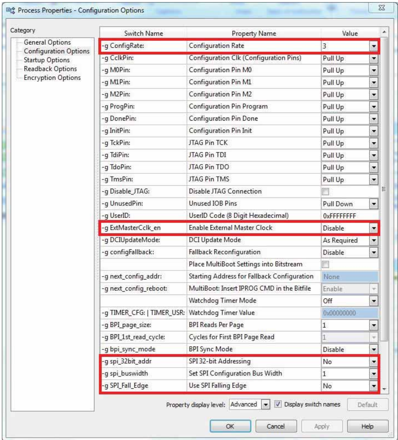
Figure 7: BitGen Configuration Options
