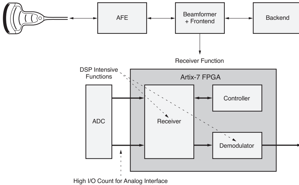
Figure 4: High DSP Performance and I/O Count for Portable Ultrasound
