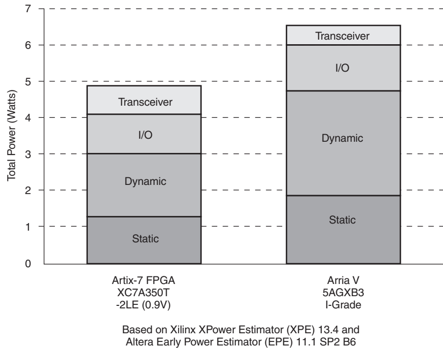
Figure 5: 34% Higher Power Consumption in Competing Device for Portable Ultrasound RX Front-End Beamformer
