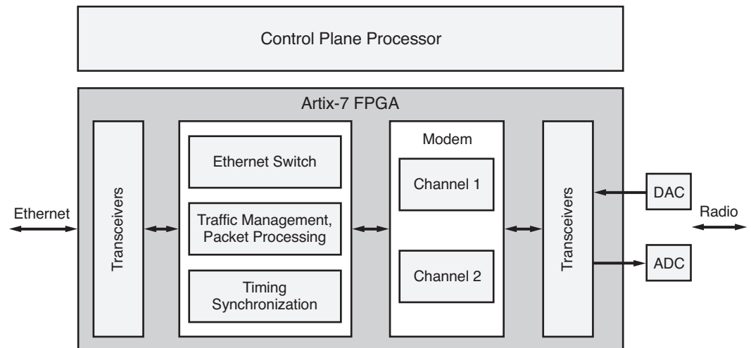
Figure 7: Integrating Multi-Device Functionality for Microwave Mobile Backhaul
